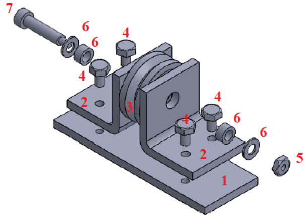
Exploded view of the Wheel Support assembly
